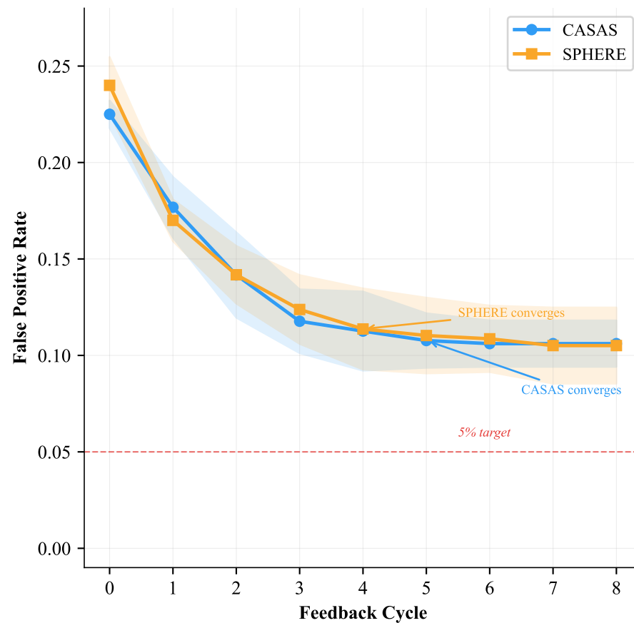
(b) False Positive Rate vs. Feedback Cycle
